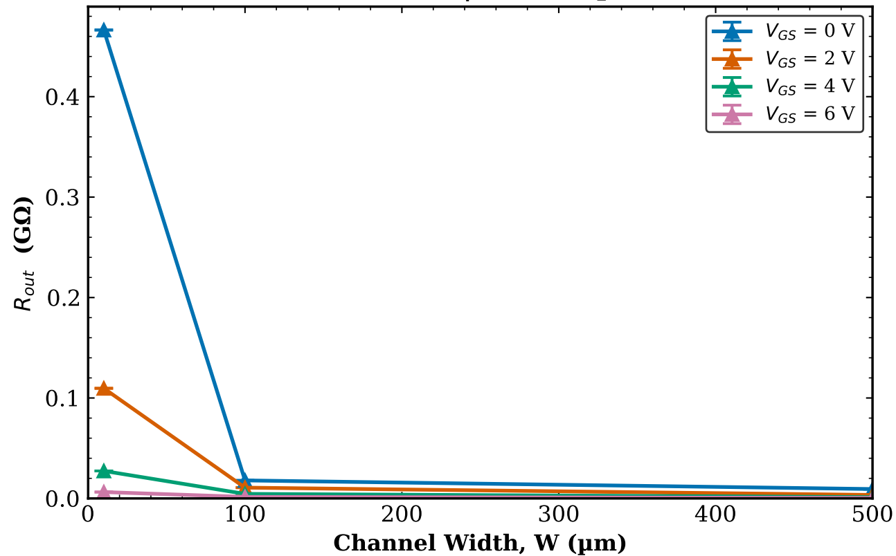
TFT1 Transistor 1 R_{out} vs W | L = 20\text{ }\mu\text{m}
